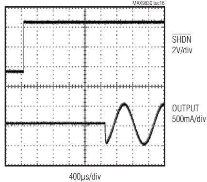
STARTUP WAVEFORM
