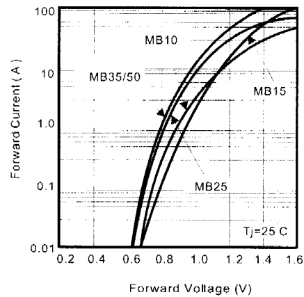
Fig. 2 - Forward Characteristics
