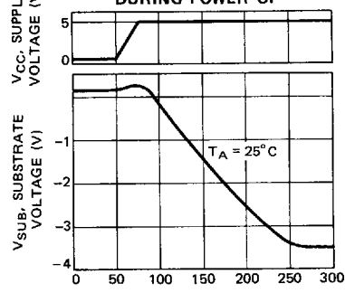
Fig. 23 – SUBSTRATE VOLTAGE DURING POWER UP
