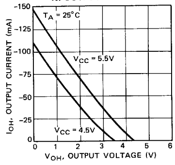
Fig. 22 – OUTPUT CURRENT vs. OUTPUT VOLTAGE
