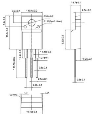
TO-220IS
