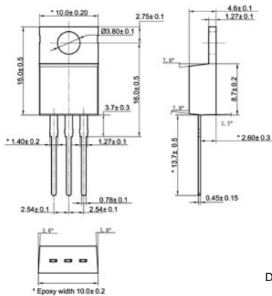
TO-220AB
