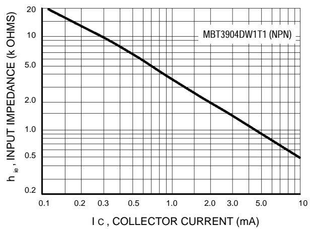
Figure 13. Input Impedance
