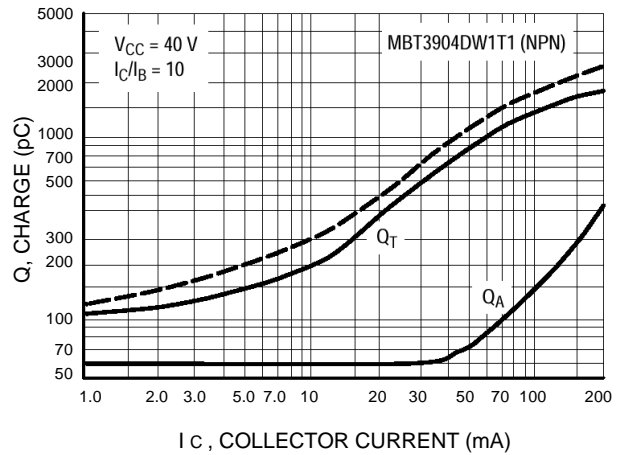
Figure 4. Charge Data
