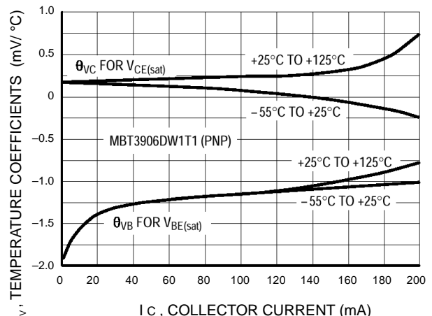
Figure 34. Temperature Coefficients
