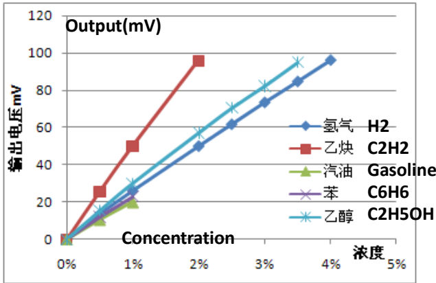
Fig3. Sensitivity Curve
