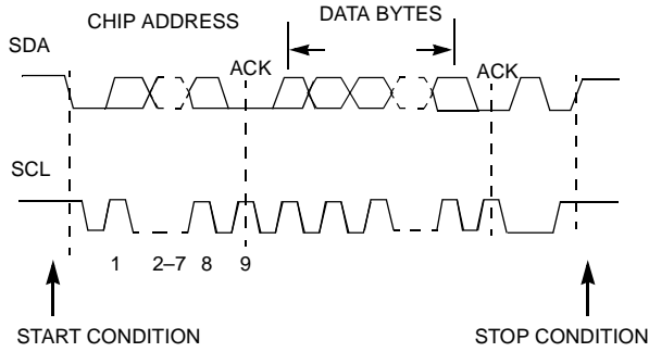
Figure 4. M-BUS Format
