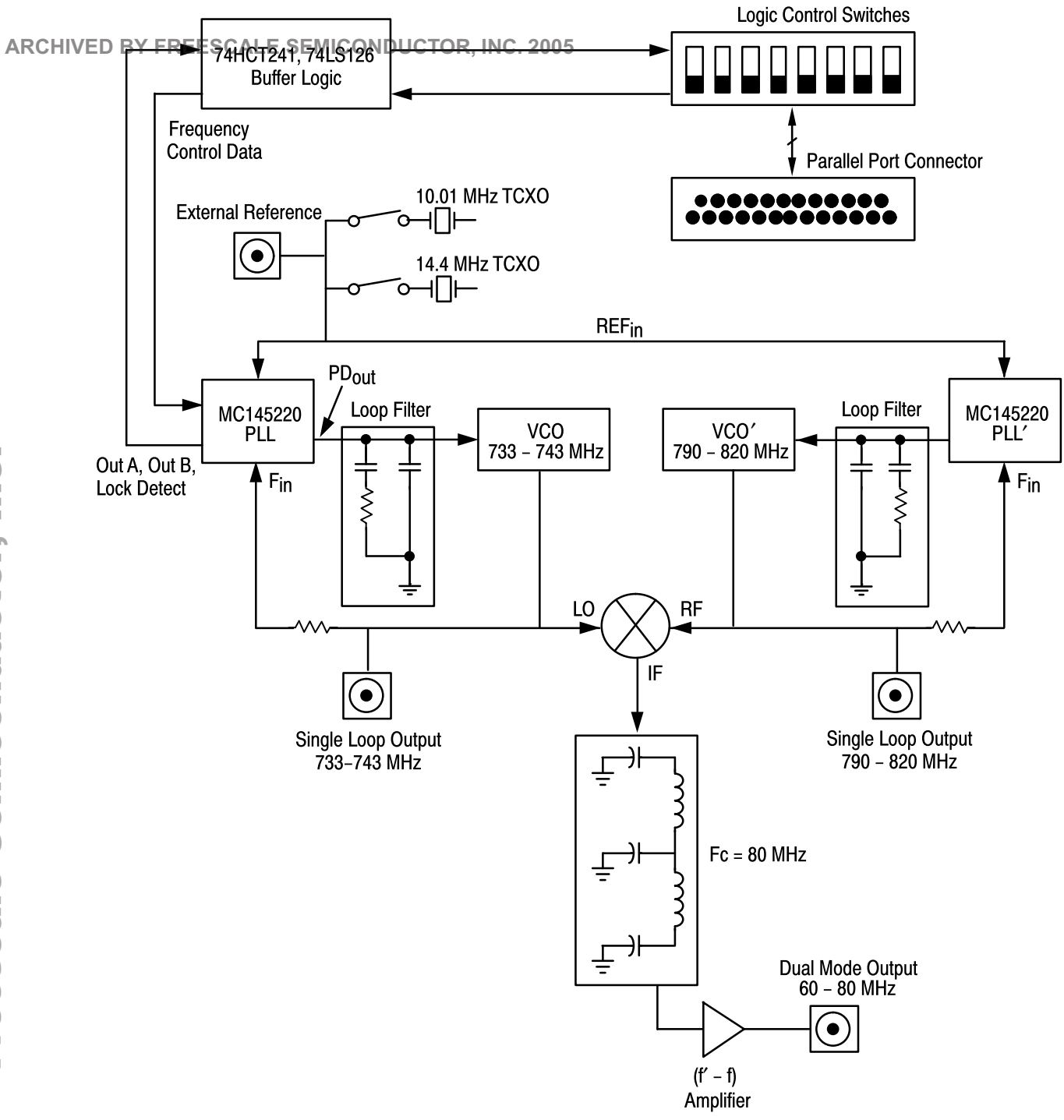
Figure 1. Evaluation Kit Block Diagram
