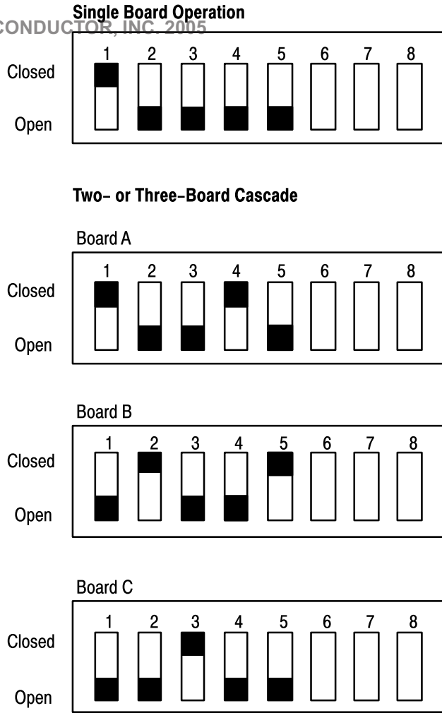
Figure 3. Switch Positions
