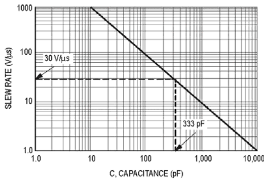
Figure 12. Slew Rate versus Capacitance for I_{SC}=10mA
