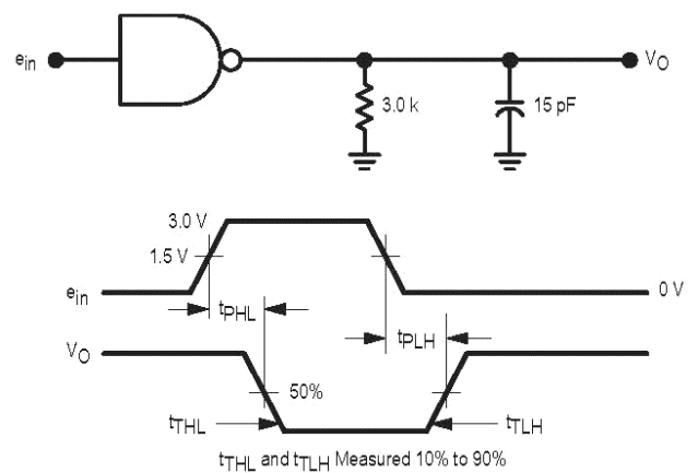
Figure 6. Switching Response
