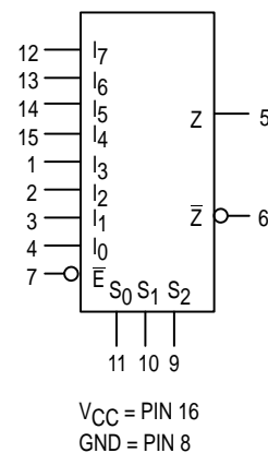
LOGIC SYMBOL
