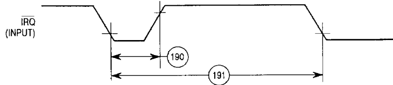
Figure 20. Interrupts Timing Diagram
