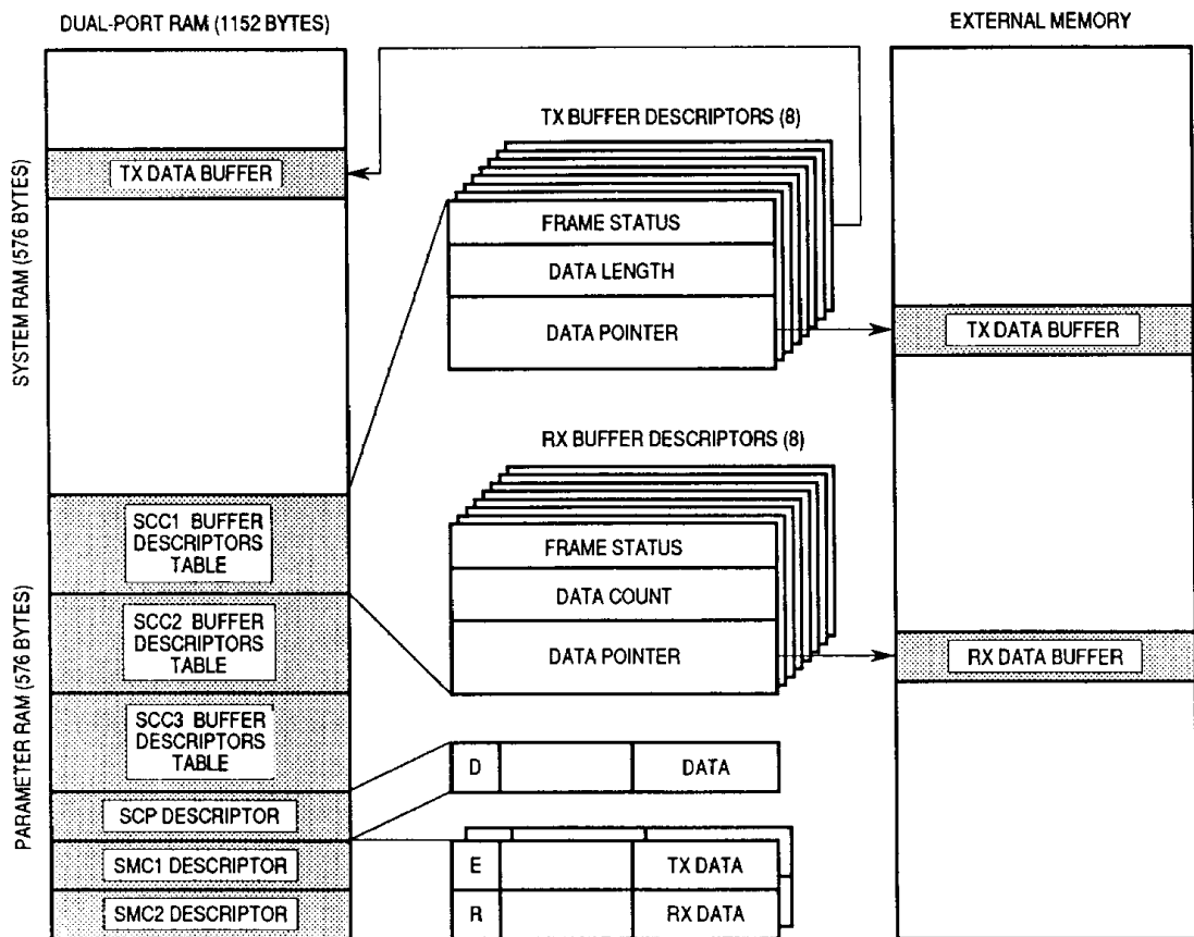
Figure 2. Buffer Memory Structure
