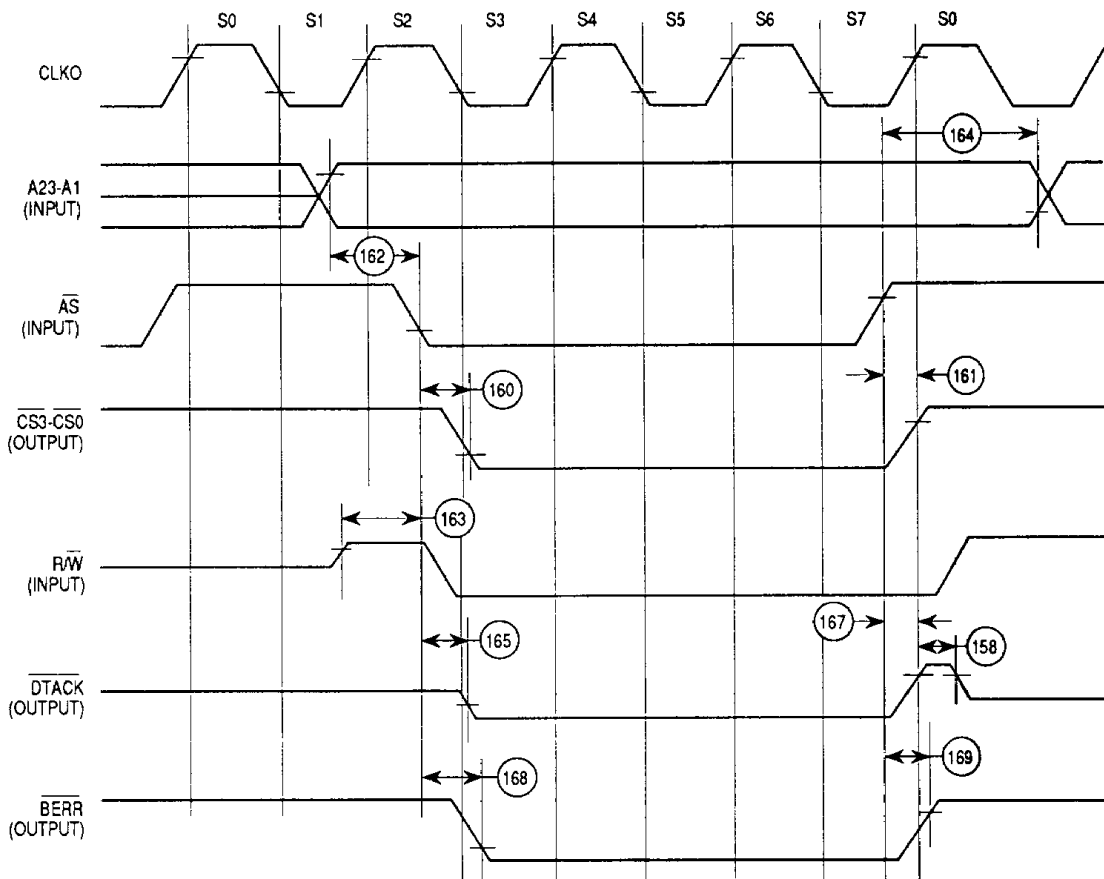
Figure 18. External Master Chip-Select Timing Diagram
