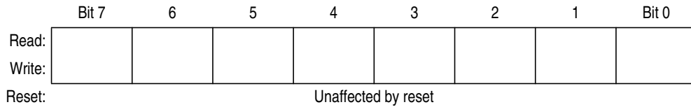
Figure 8-2. Accumulator (A)
