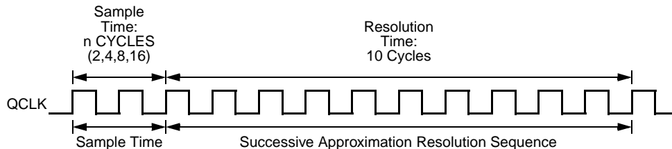
Figure 28-21. Bypass Mode Conversion Timing
