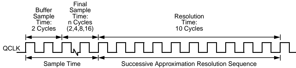
Figure 28-20. Conversion Timing
