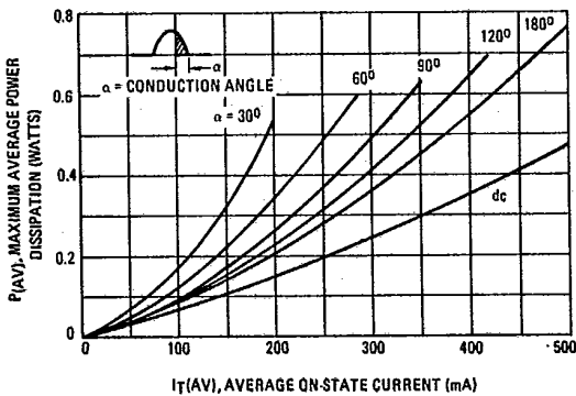
FIGURE 2 - POWER DISSIPATION
