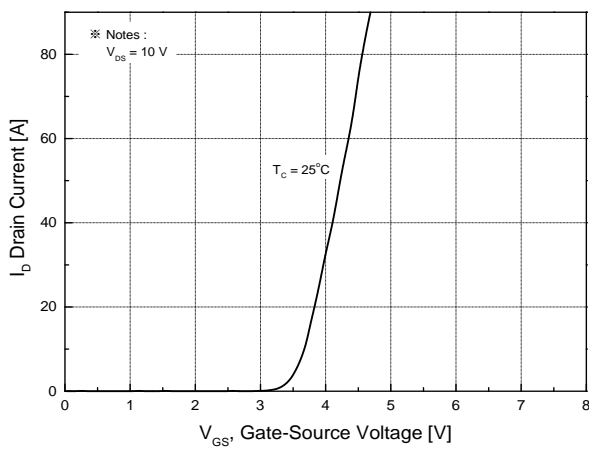
Fig.5 Transfer Characteristics
