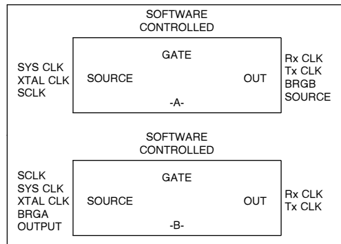
Figure 11. BRG Sources and Outputs
