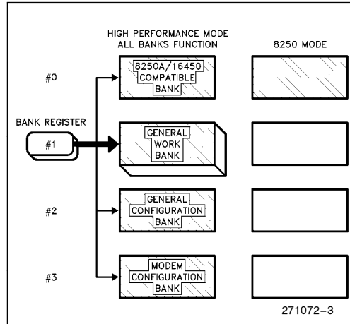
Figure 3. M82510 Register Architecture
