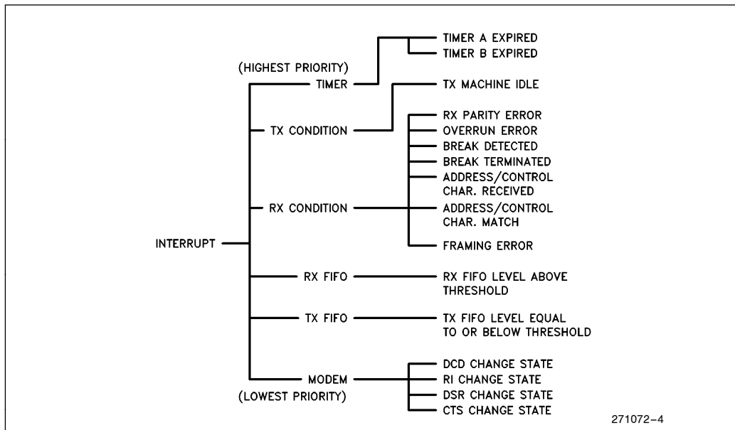
Figure 4. Interrupt Structure
