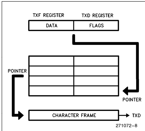
Figure 8. Tx FIFO
