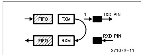
Figure 12. Local Loopback
