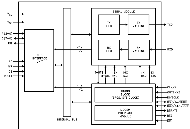
Figure 1. Block Diagram
