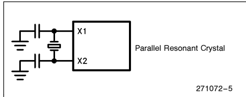
Figure 5. Crystal Oscillator
