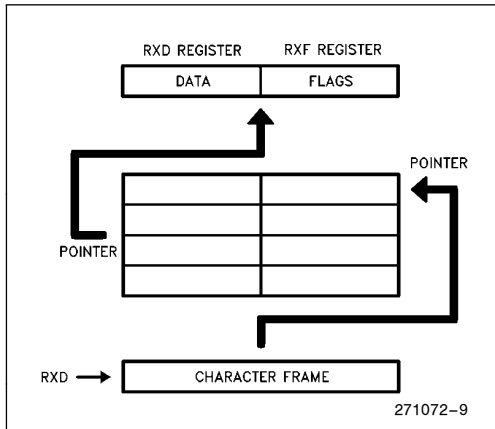
Figure 9. Rx FIFO
