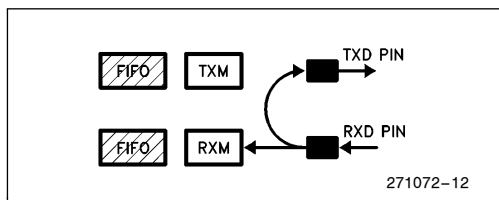
Figure 13. Remote Loopback
