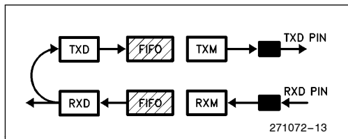
Figure 14. Auto Echo
