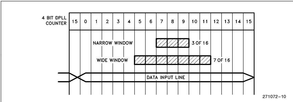
Figure 10. Sampling Windows
