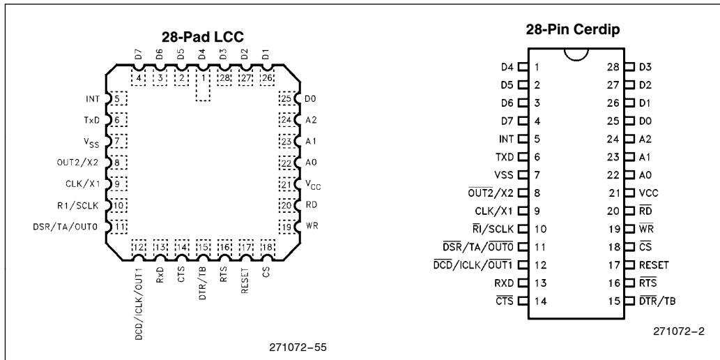
Figure 2. Package Pinouts
