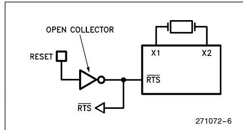
Figure 6. Strapping Option
