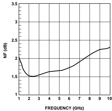
Figure 3. Matched Noise Figure vs. Frequency.
