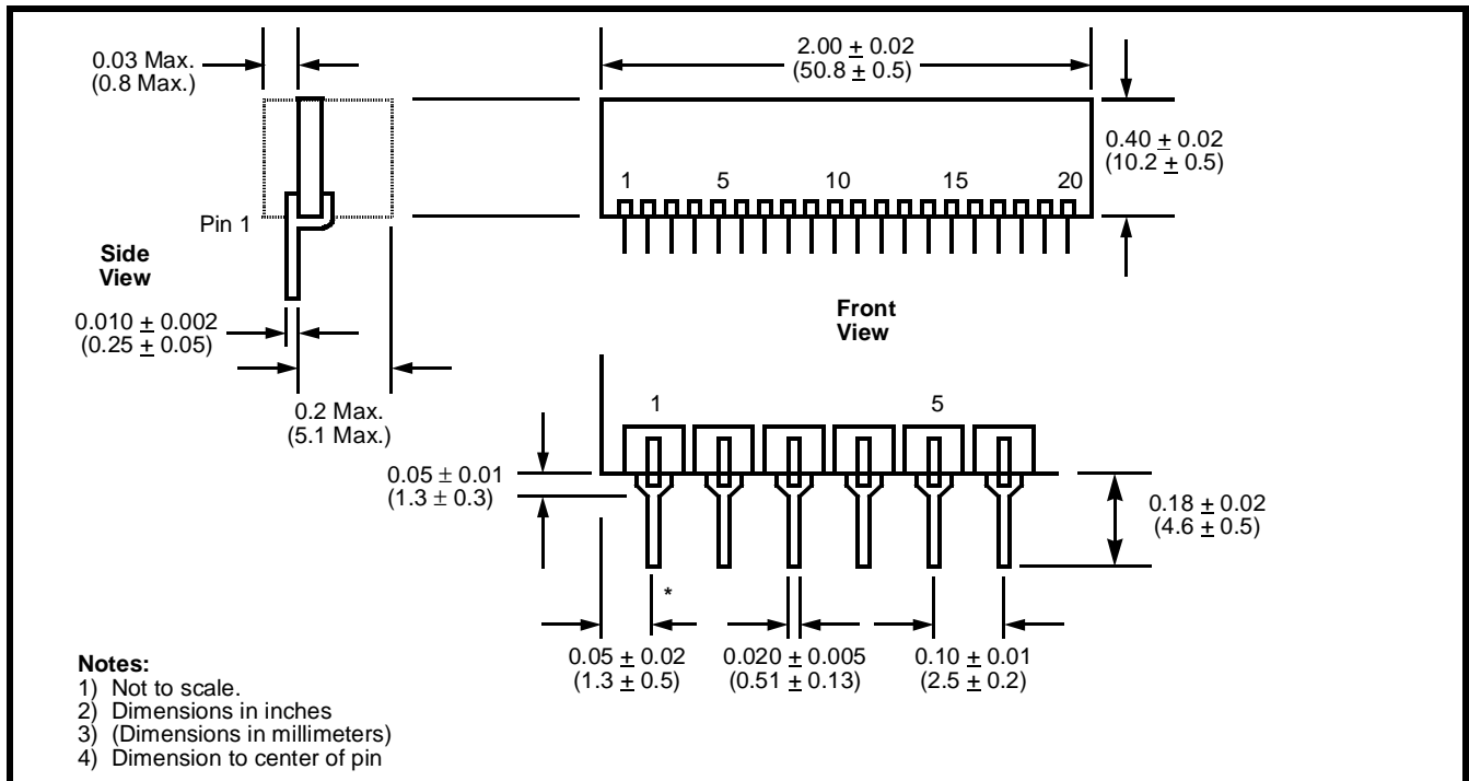
Figure 4 - Mechanical Data
