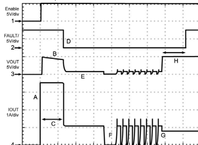
Figure 3. Kickstart™ Operation
