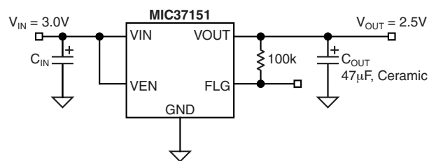
Fixed 2.5V Regulator with Error Flag
