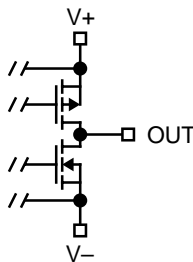
MIC7211 Push-Pull Output
