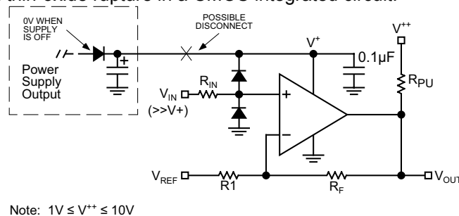
Figure 2. Avoid This Condition
