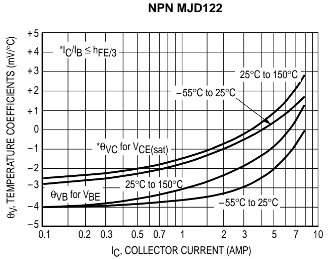
Figure 5. Temperature Coefficients
