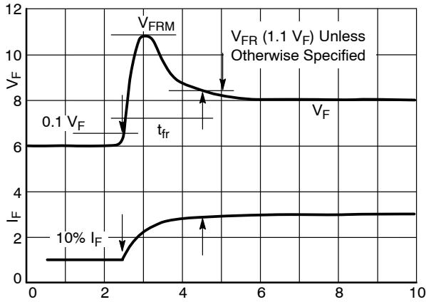
Figure 26. t_{rr} Measurement
