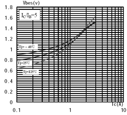
V bes -I C
