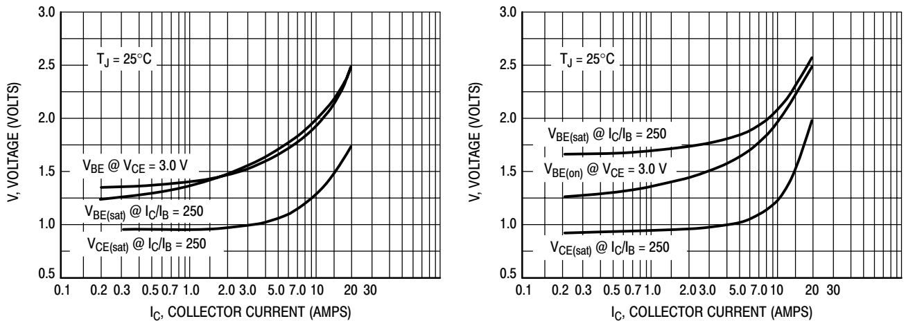
Figure 9. "On" Voltages
