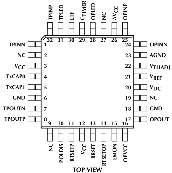
ML4664/ML4669 32-Pin TQFP (H32-7)
