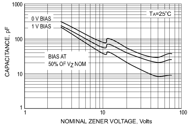
Fig.4 TYPICAL CAPACITANCE
