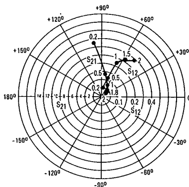
FORWARD/REVERSE TRANSMISSION COEFFICIENTS versus FREQUENCY V CE = 5 V, I C = 30 mA
