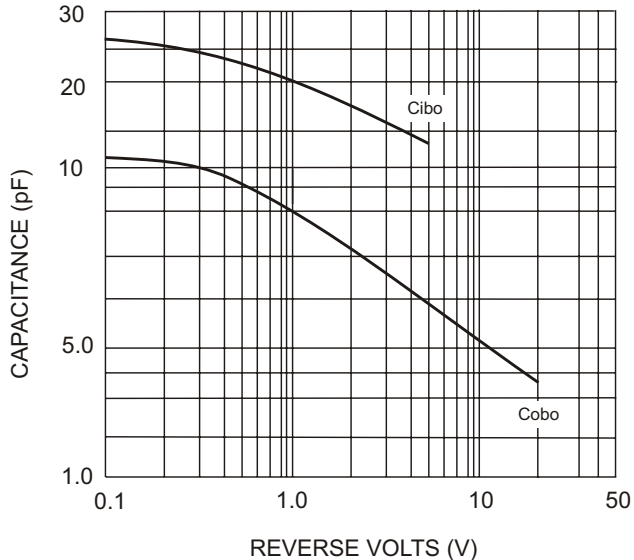
Fig. 3 Typical Capacitance
