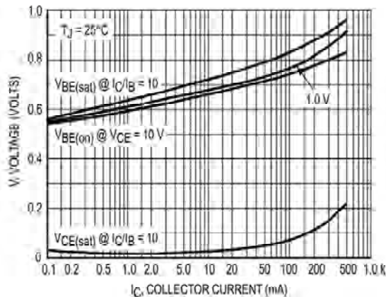
"On" Voltages
