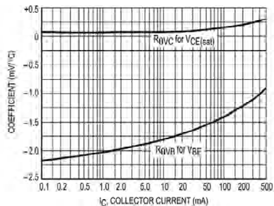
Temperature Coefficients
