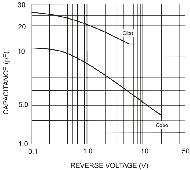
Fig. 3 Capacitances (Typical)
