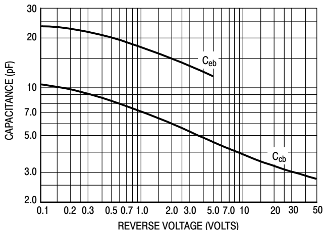
Figure 9. Capacitances
