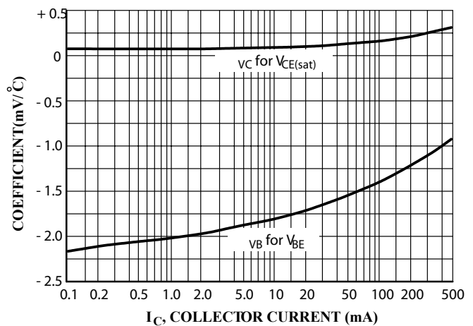
Figure 18. T emperature Coefficients
