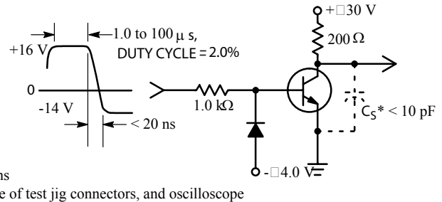
Figure 2. Turn-Off Time
