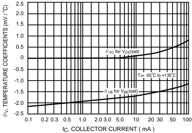
Figure 5. Temperature Coefficients
