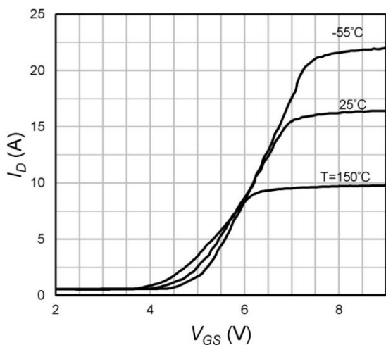
Fig.5 Transfer Characteristics
