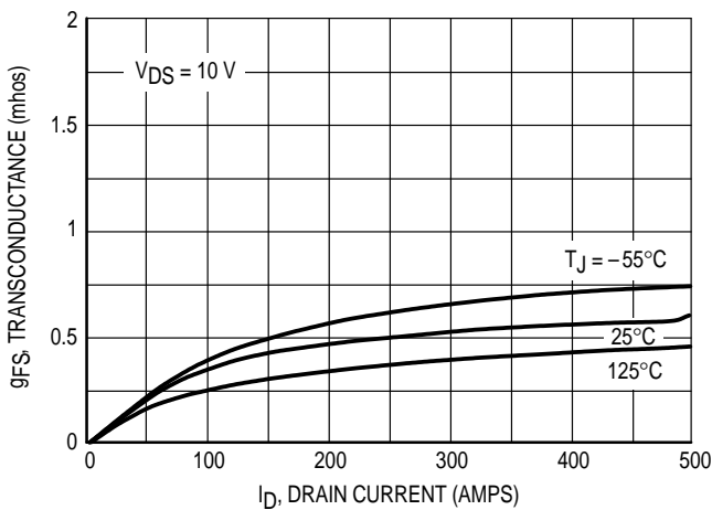
Figure 8. Transconductance
