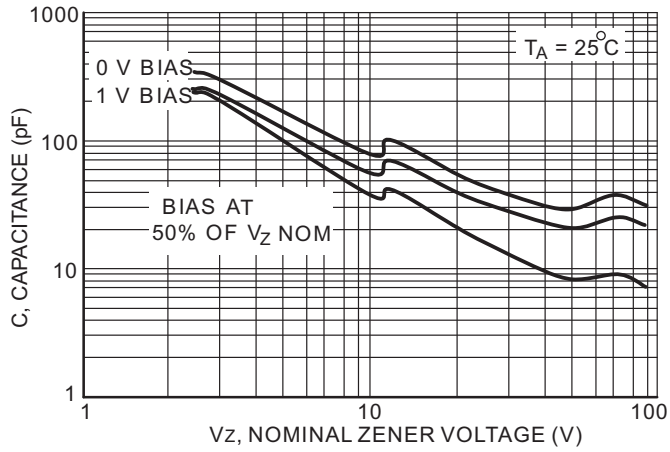
FIG7. Typical Capacitance
