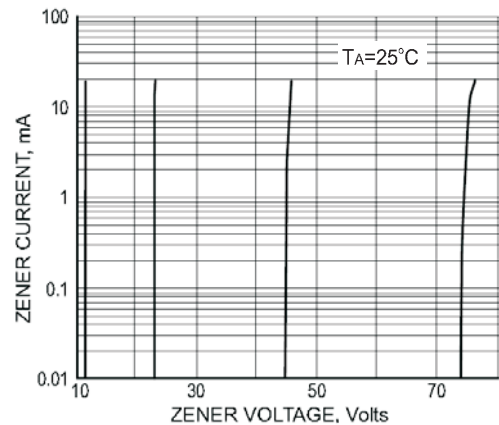
FIG. 6-ZENER BREAKDOWN CHARACTERISTICS
