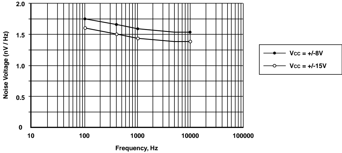
Noise as a Function of Frequency
