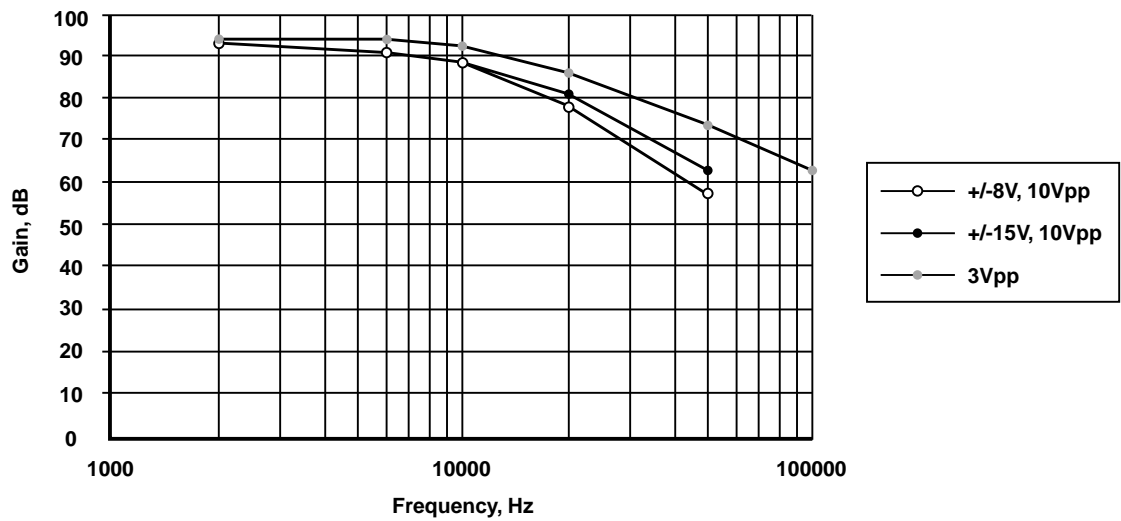
Total Harmonic Distortion, MN2311
