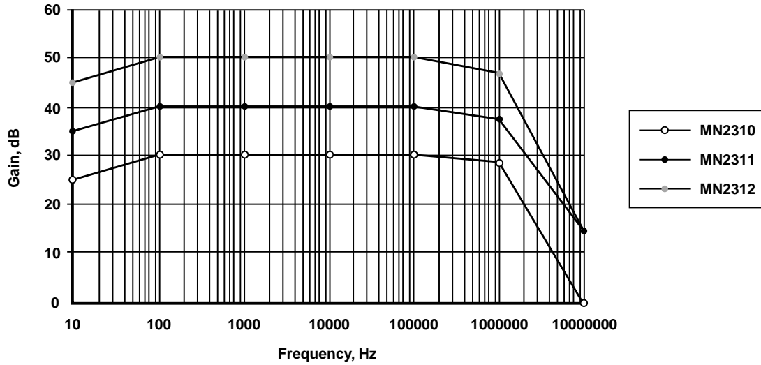
Frequency Response
