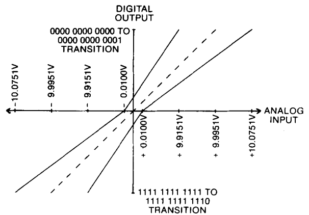
MN5202H ABSOLUTE ACCURACY -55^\circ C AND +125^\circ C
