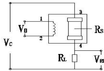
Fig2.Test circuit for MP-4
