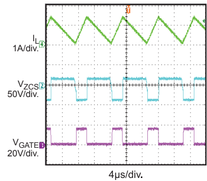
Zero-current Sensing
