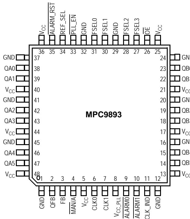
Figure 2. MPC9893 48-Lead Pinout (Top View)
