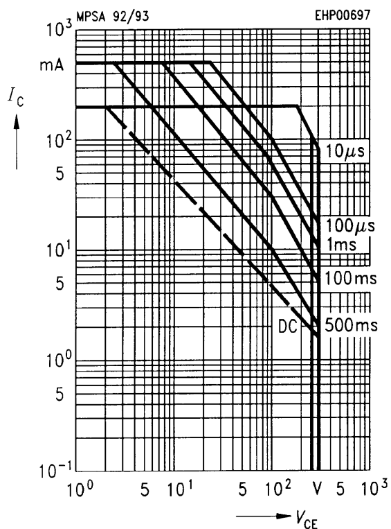
Operating range I_c = f(V_{CE0}) T_A = 25^\circ\text{C}, D = 0
