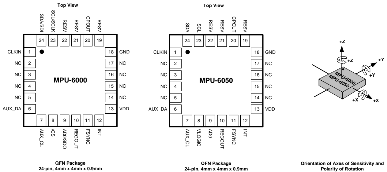
Figure 2. MPU-6000 QFN Package (Top View) 24-pin 4mm x 4mm x 0.9mm & Axis Orientation
