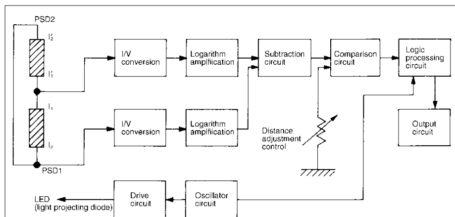
Fig. 5 Signal processing circuit block diagram
