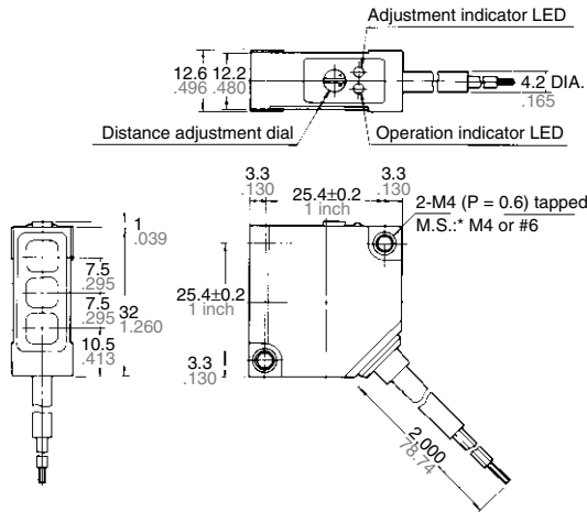
Outline dimensions
