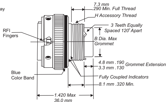
Plug Shell, RFI Grounding, Bayonet Coupling Military No. MS3475 Amphenol No. MB18
