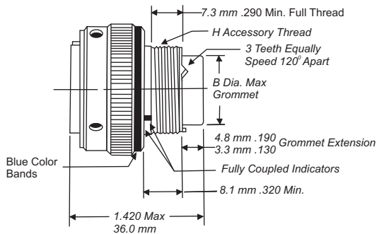
Plug Shell, Bayonet Coupling Military No. MS3476
