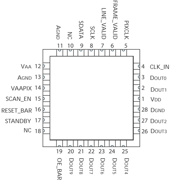
Figure 3: Pin Out Diagram - 28-Pin PLCC
