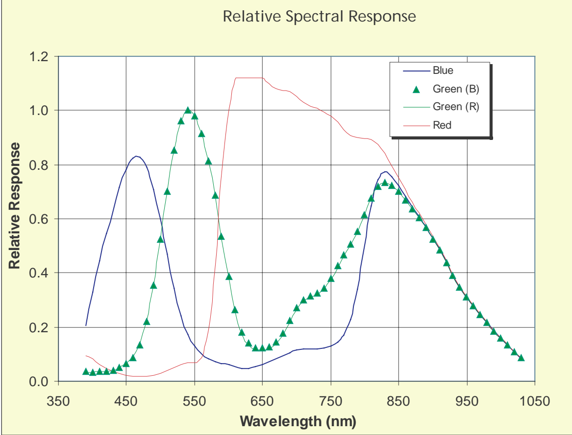
Figure 28: Spectral Response
