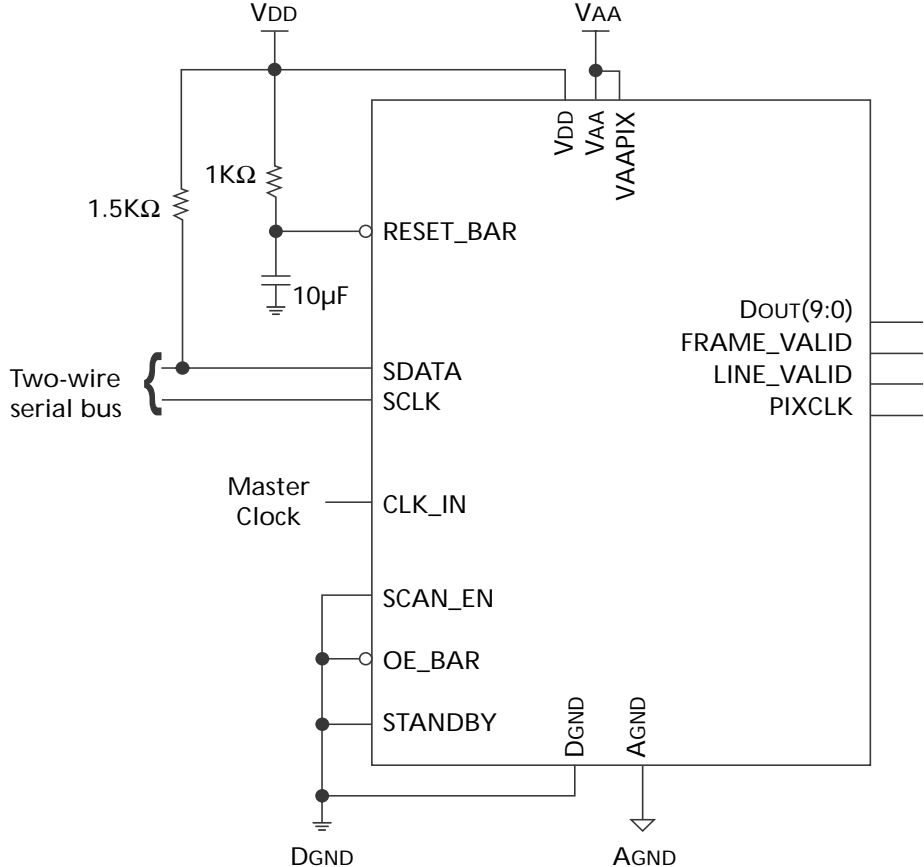
Figure 2: Typical Configuration (Connection)
