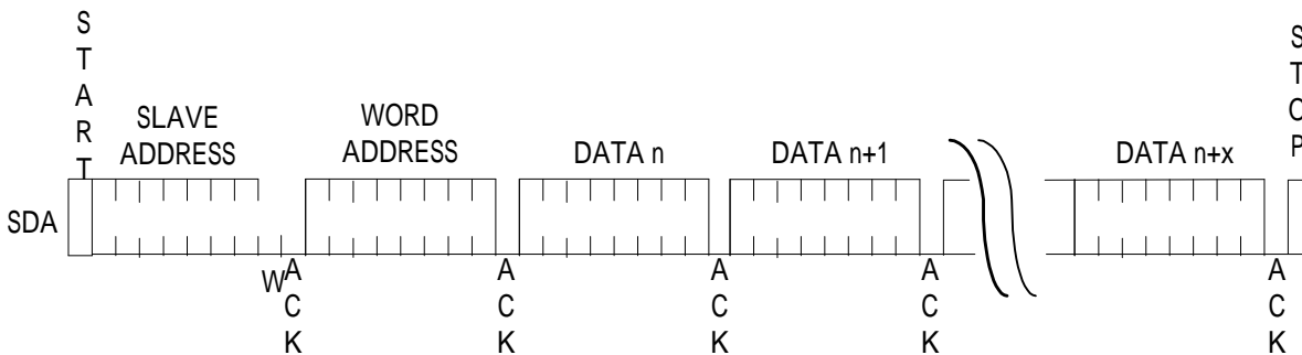
Fig. 3.5.3 Sequential Write
